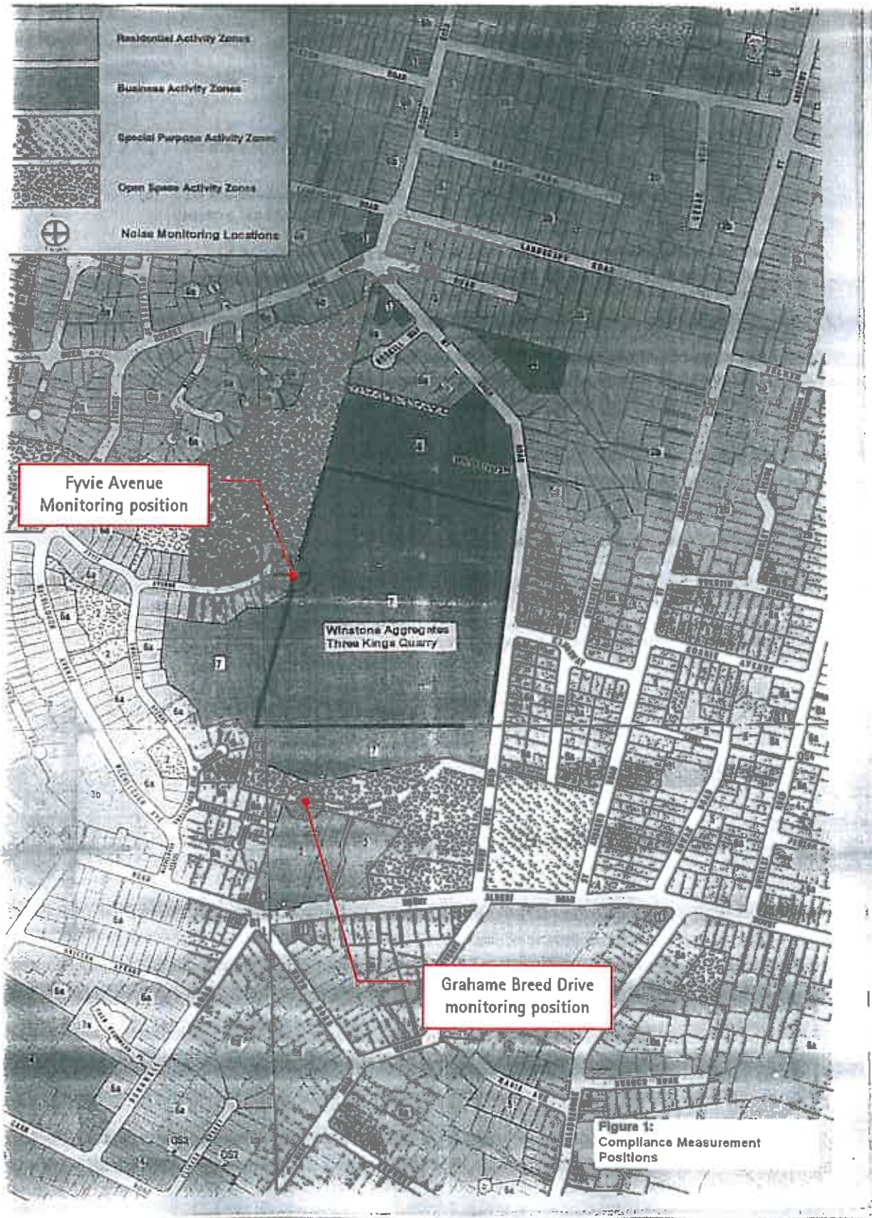
FIGURE 1 – MEASUREMENT POSITIONS
